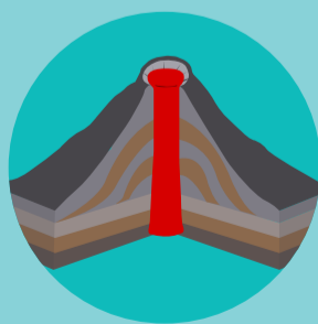
CINDER CONE VOLCANO
