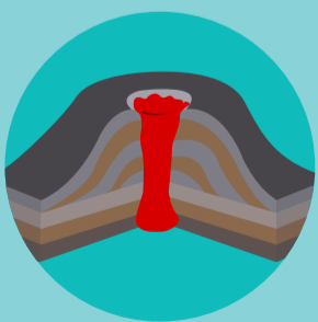
LAVA DOME VOLCANO
